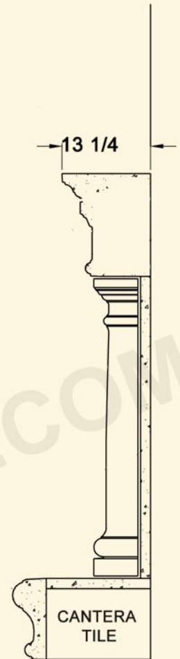
SIDE SECTION
